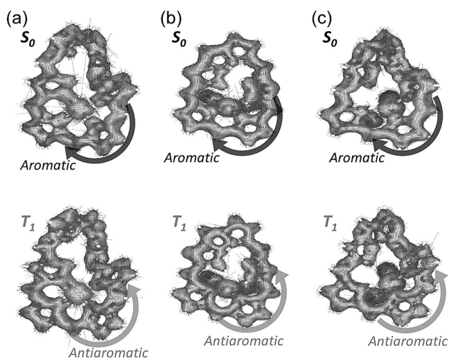
Figure 5. ACID plots of a) Pd28H, b) Rh22P, and c) Rh24P in the ground (top) and triplet (bottom) states. Hydrogen atoms and meso-pentafluorophenyl groups omitted for clarity. For magnified images, see Figures S14–S16.
